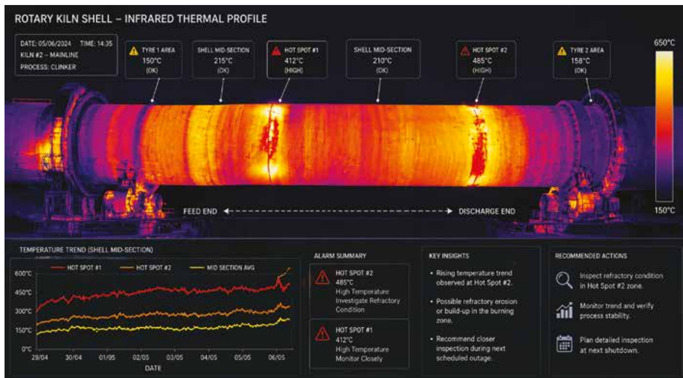
Figure 2: Infrared shell temperature profile rotary kiln predictive maintenance.
