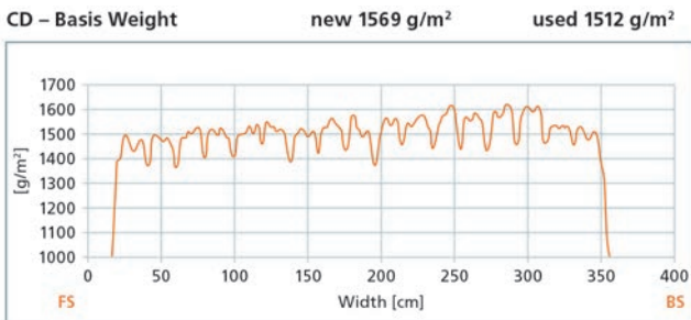
Fig. 13: Zonal felt wear recognizable in the basis weight profiles taken from the removed felt
